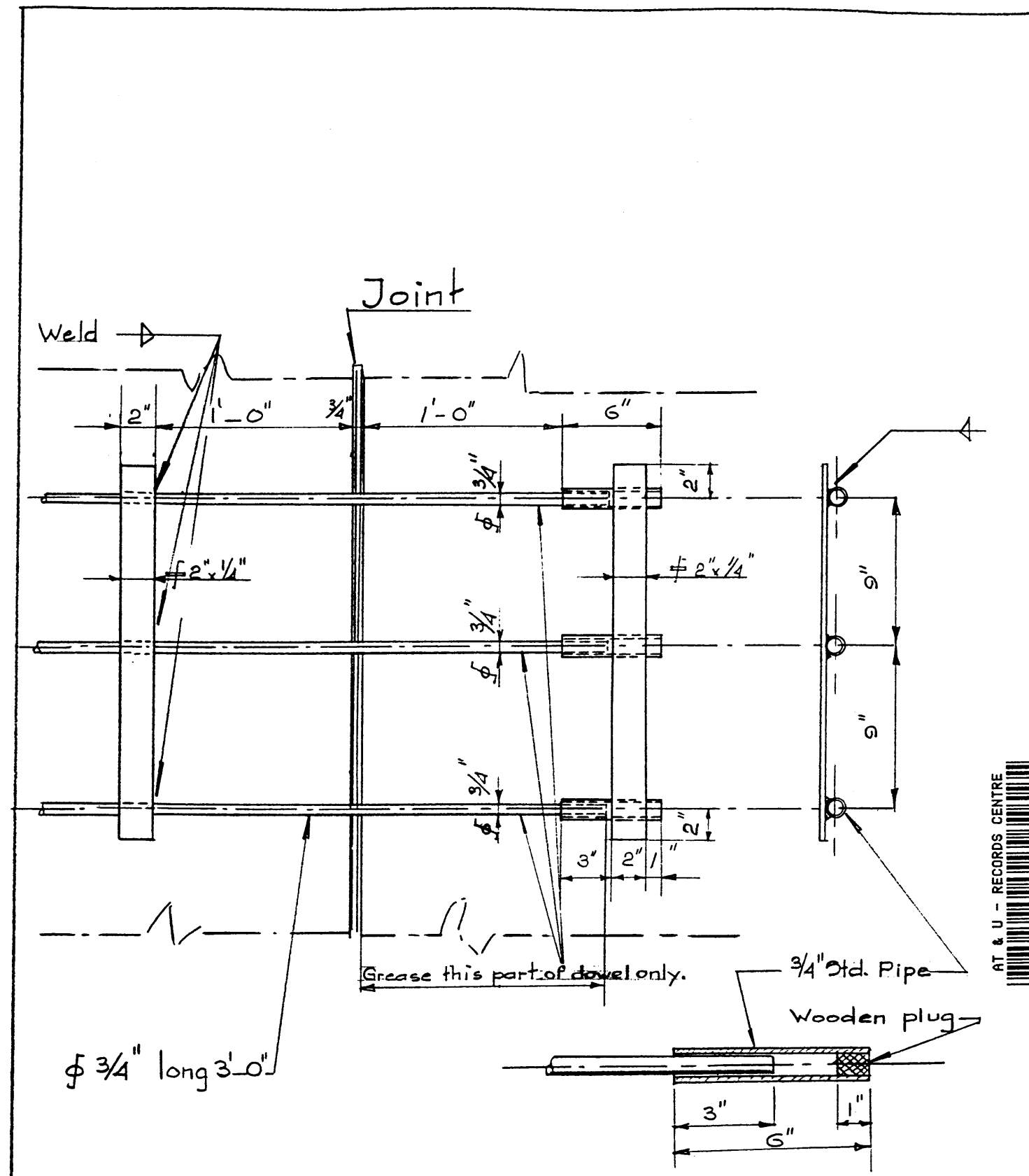
Sliding Dowel Joint
