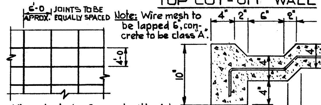
TOP CUT-OFF WALL
