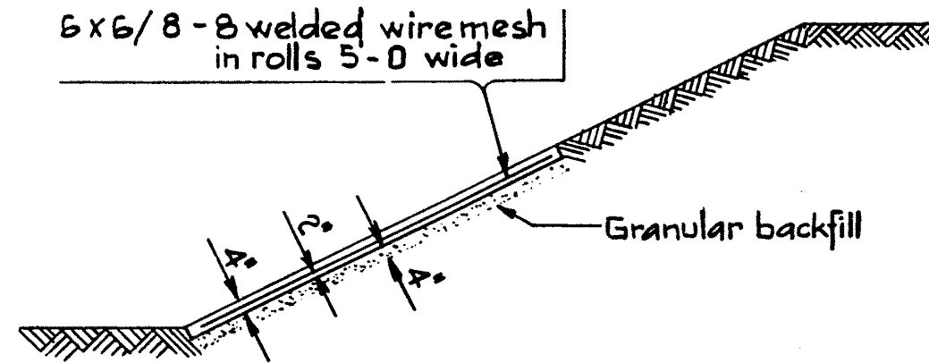
WITHOUT TOP OR TOE CUT-OFF WALLS.
