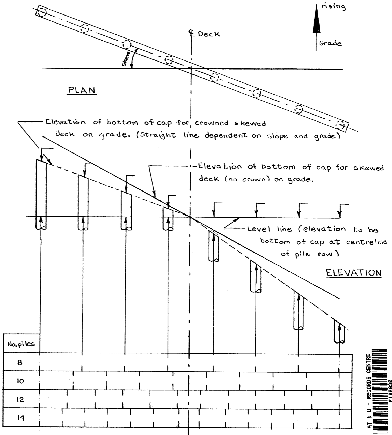
PILE CUT OFFS FOR SKEWED CROWNED RDWY. ON GRADE
