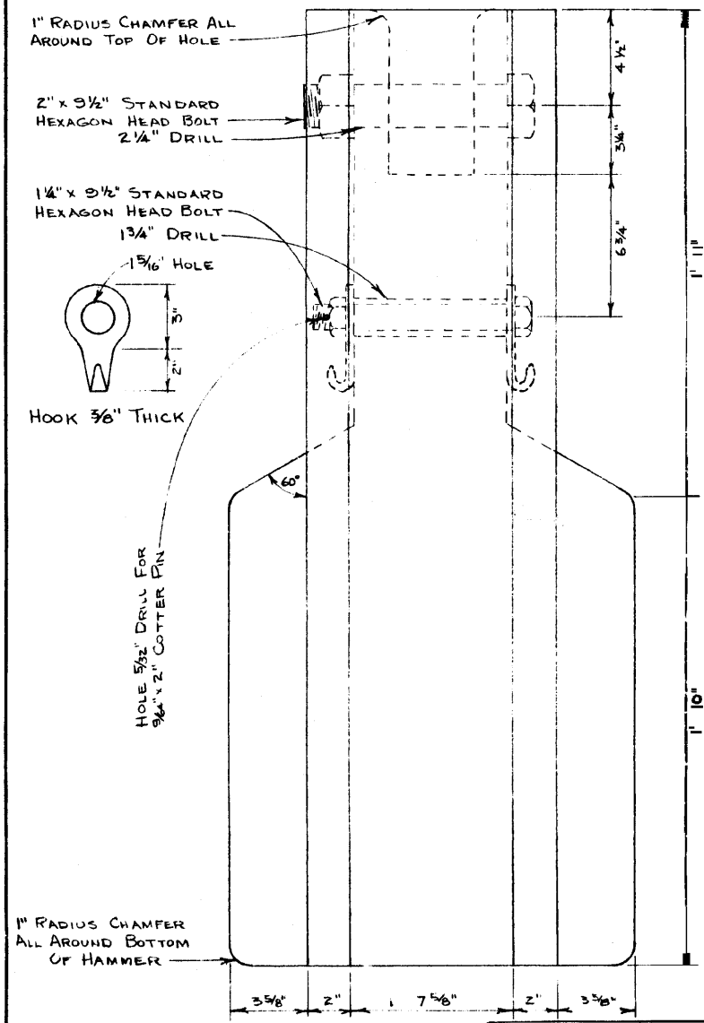
SIDE VIEW PILE HAMMER
