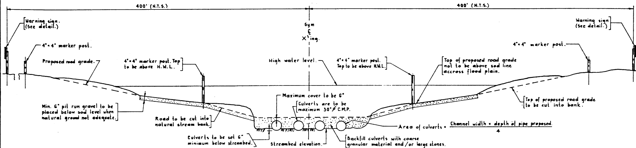
SECTION A-A Cross section of crossing along road.
