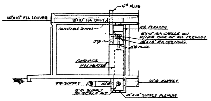
SECTION A 1/4"=1'-0"
