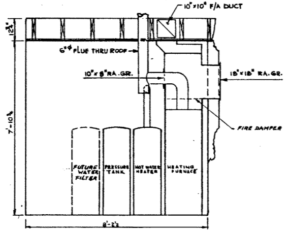
SECTION B 1/2"=1'-0"
