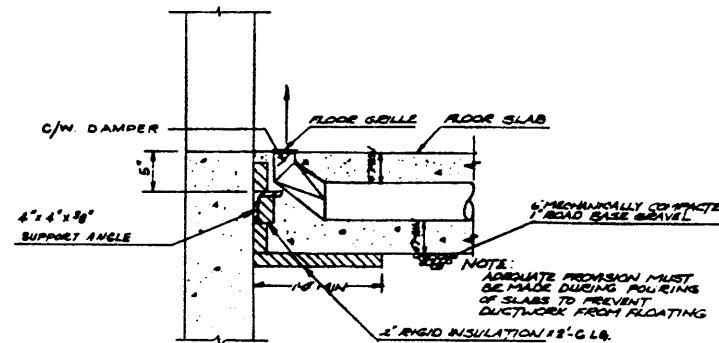
B SECTION 1/75
