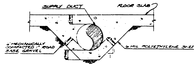
C SECTION 1/75
