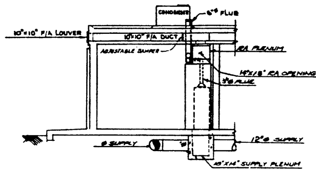
A SECTION 1/4" = 1'-0"
