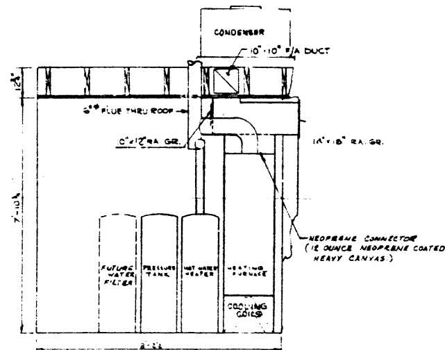
D SECTION 3/16"
