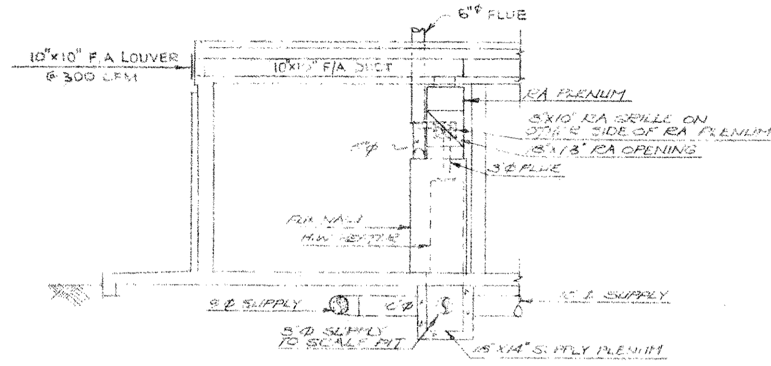
A SECTION SCALE 1/2"=1'-0"
