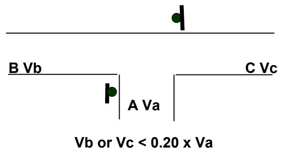
Figure 1 – Non-conventional installation of Stop signs at a “T” intersection.
