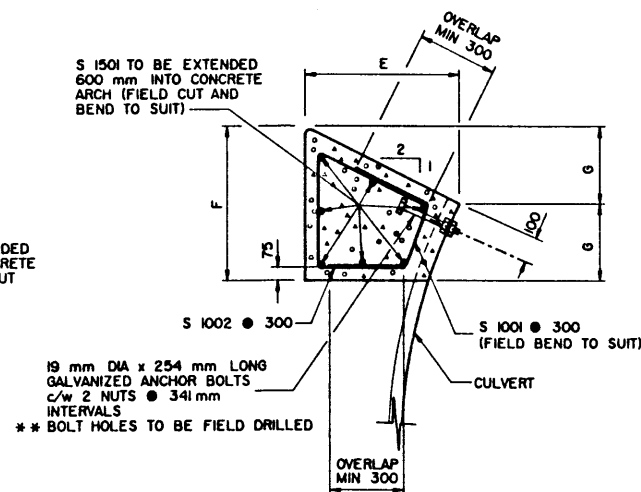
SECTION - SHOULDER
