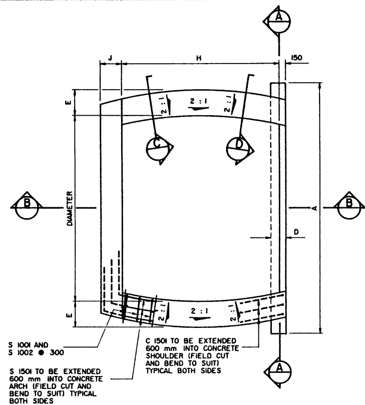
PLAN VIEW OF CONCRETE COLLAR
