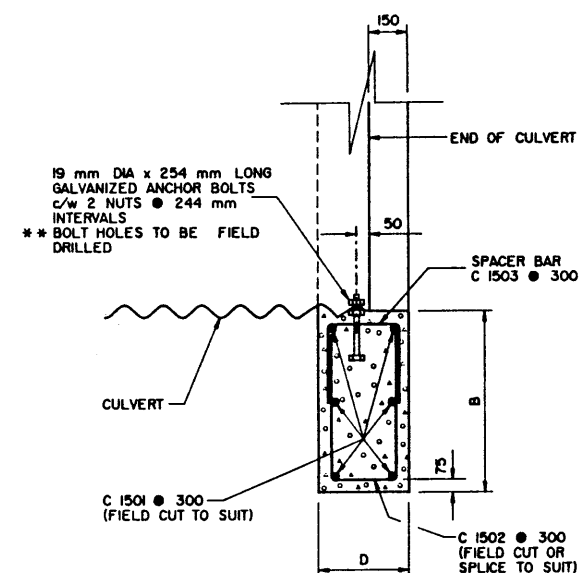
DETAIL - CUT-OFF
