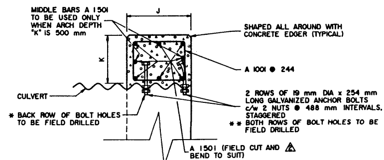
DETAIL - ARCH
