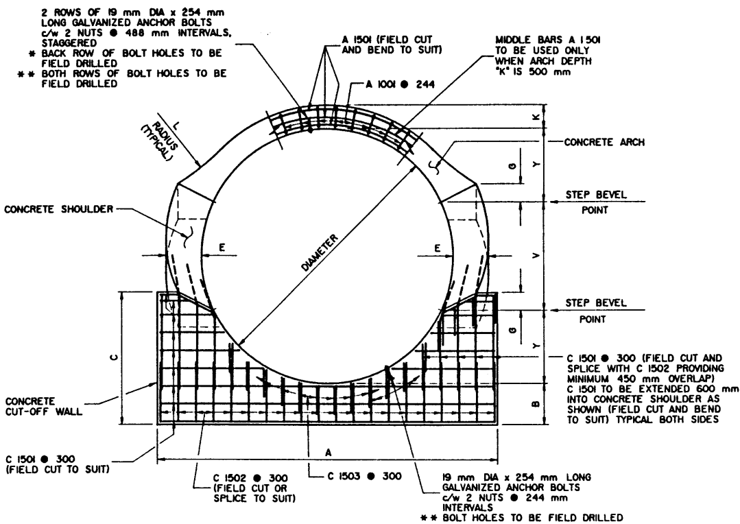
SECTION - END VIEW
