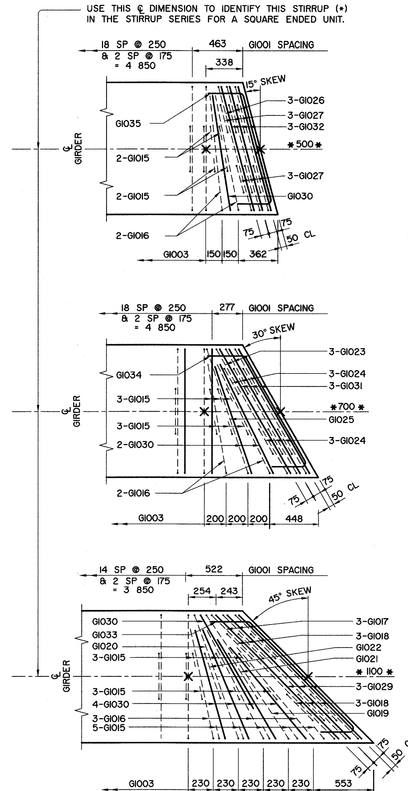
SKREW GIRDER END REINFORCING BARS
