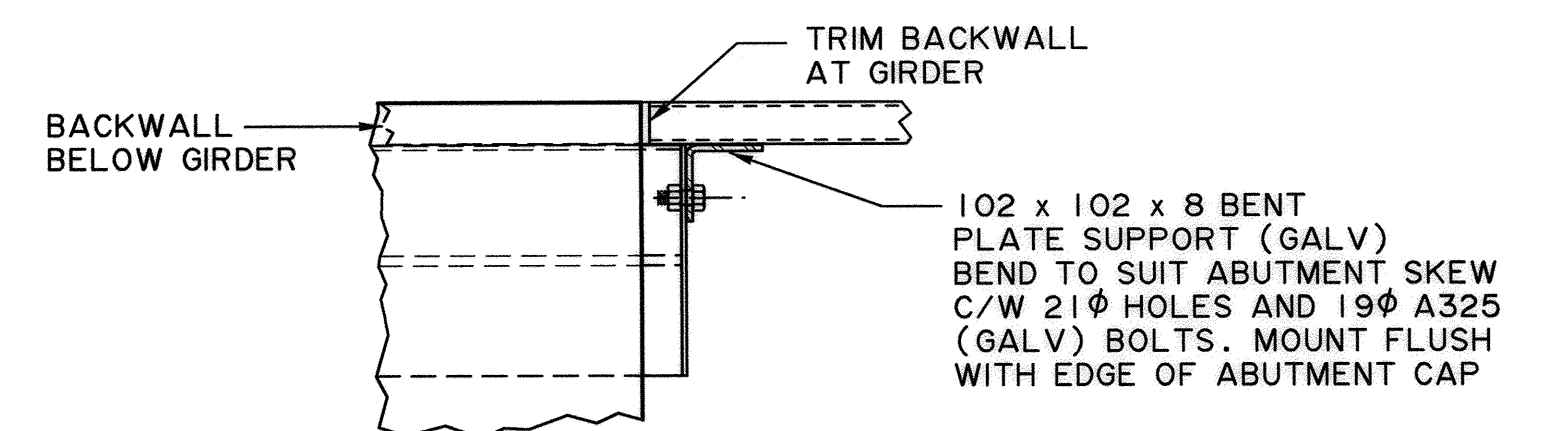
DETAIL - WINGWALL PILE S-1753 1:5
