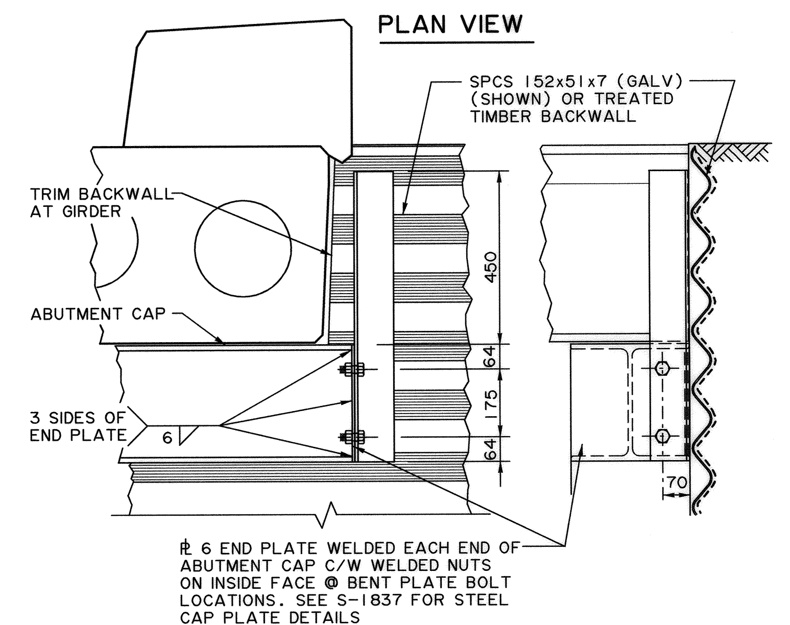
CAP PLATE DETAILS ELEVATION END VIEW 2 W DETAIL - BACKWALL SUPPORT ANGLE S-1755 (SLW GIRDER BRIDGES ONLY) 1:10
