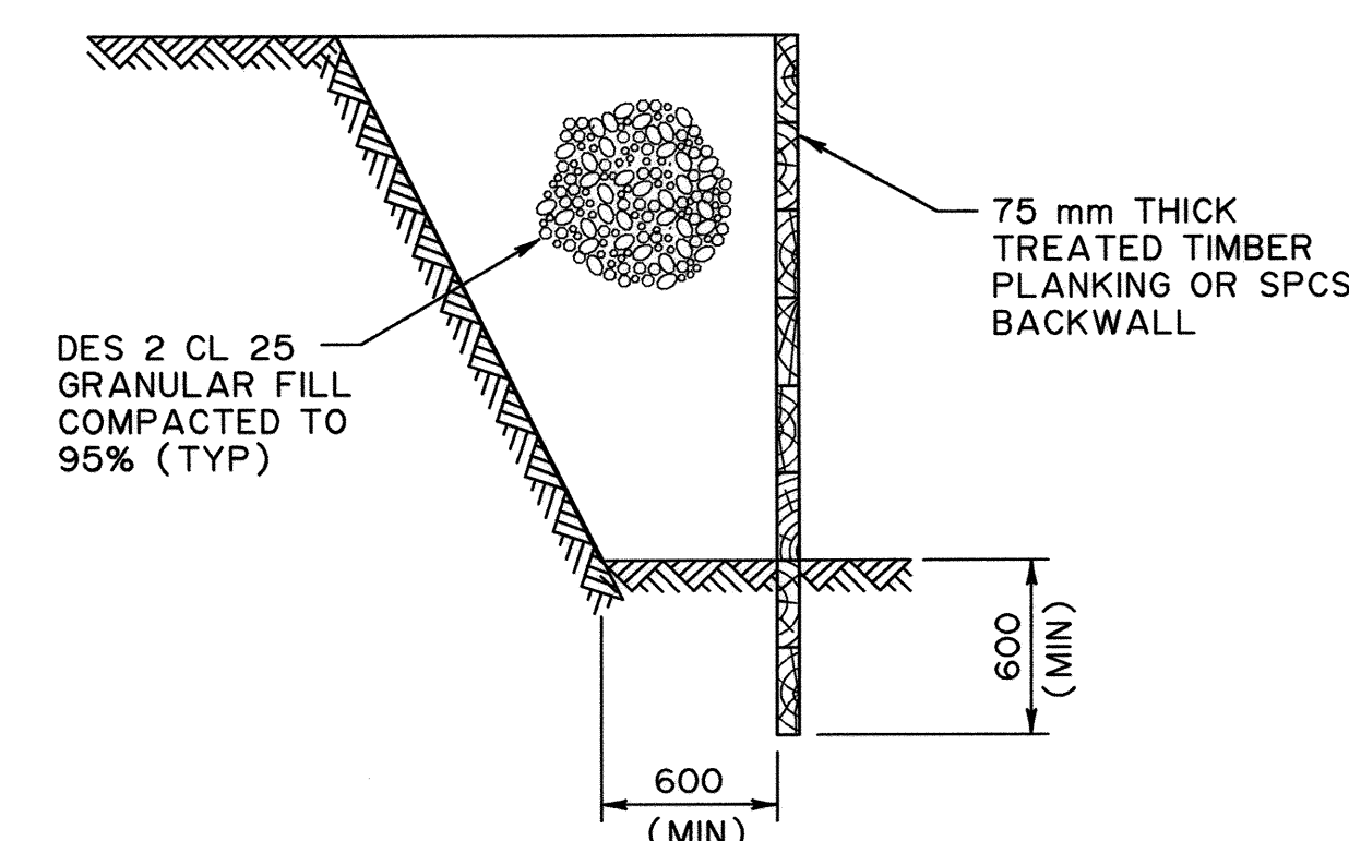
BACKFILL DETAIL
