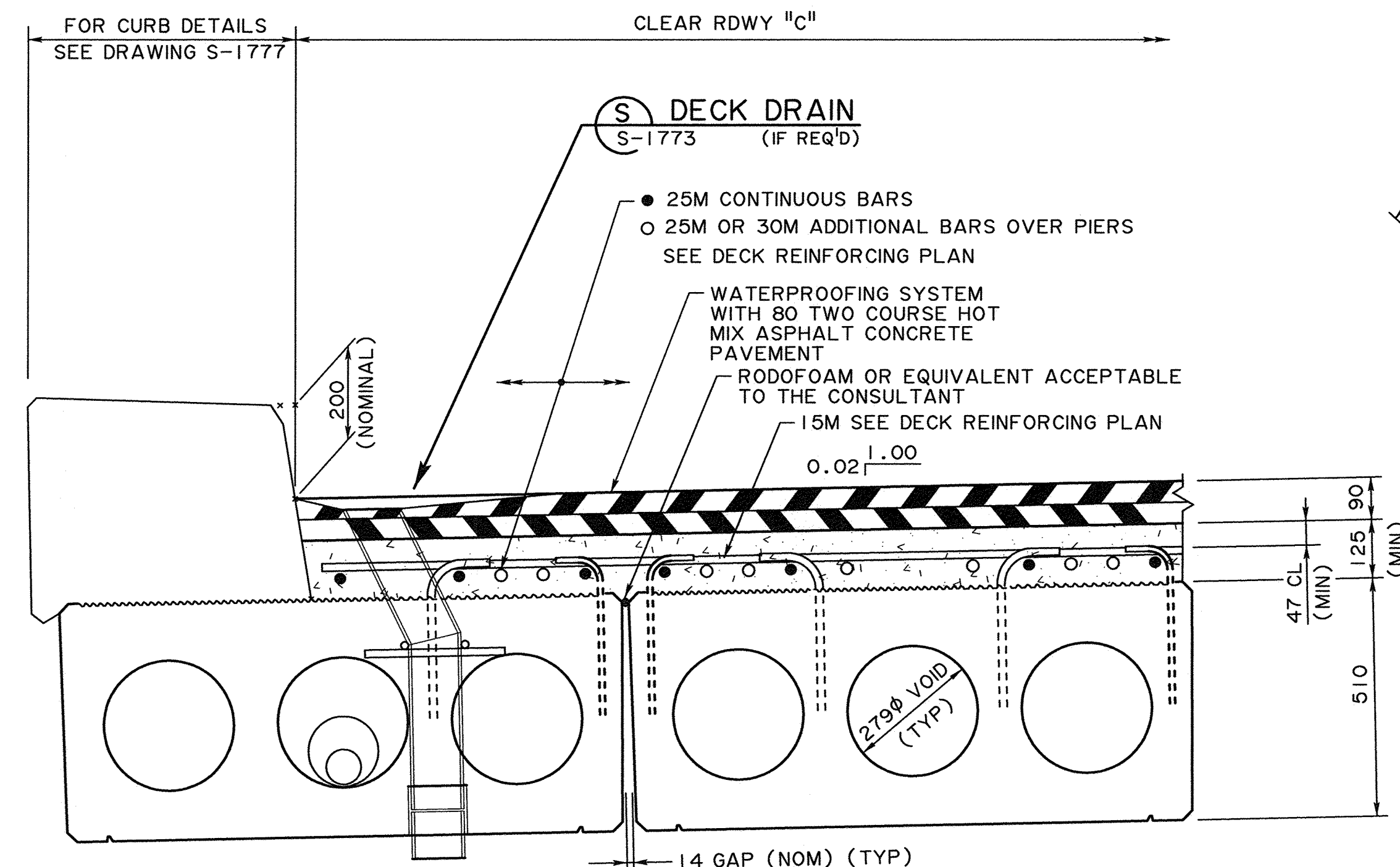
TYPICAL DECK SECTION S-1771 (FOR ACP WEARING SURFACE) 1:10
