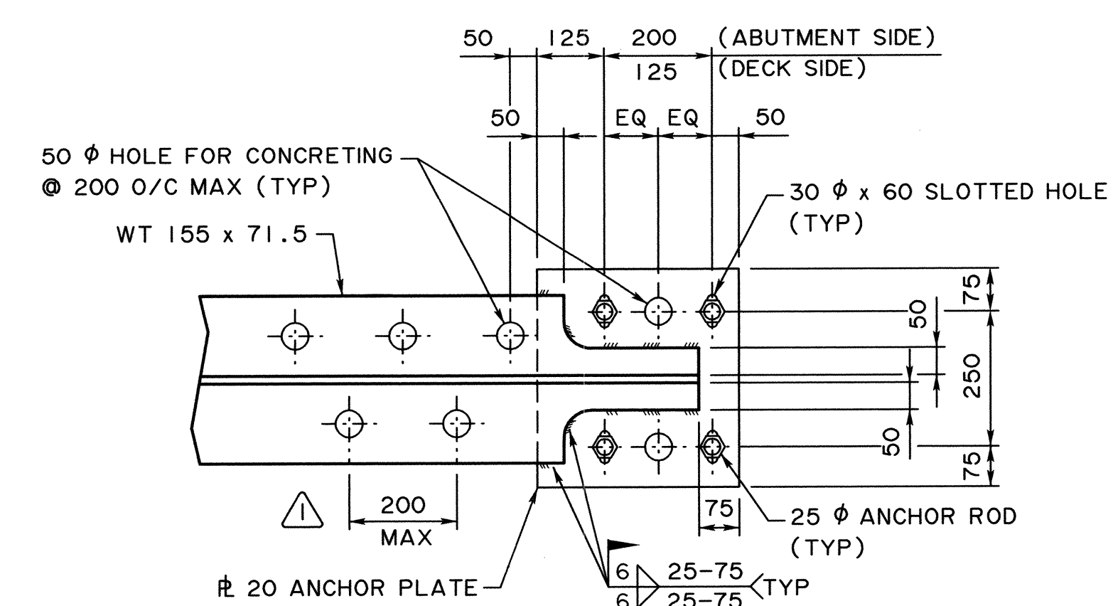
WT STIFFENER AND ANCHOR ROD ASSEMBLY
