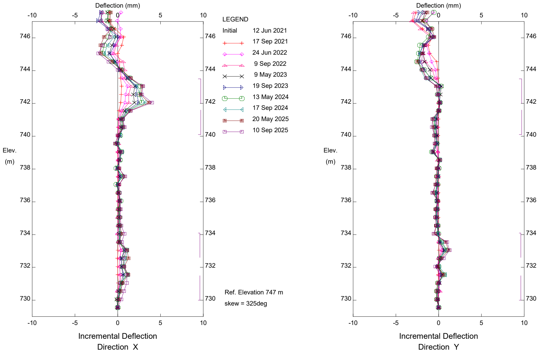
C017-III; H575:04; Truckstop Slide, Inclinator SI20-01 Alberta Transportation
