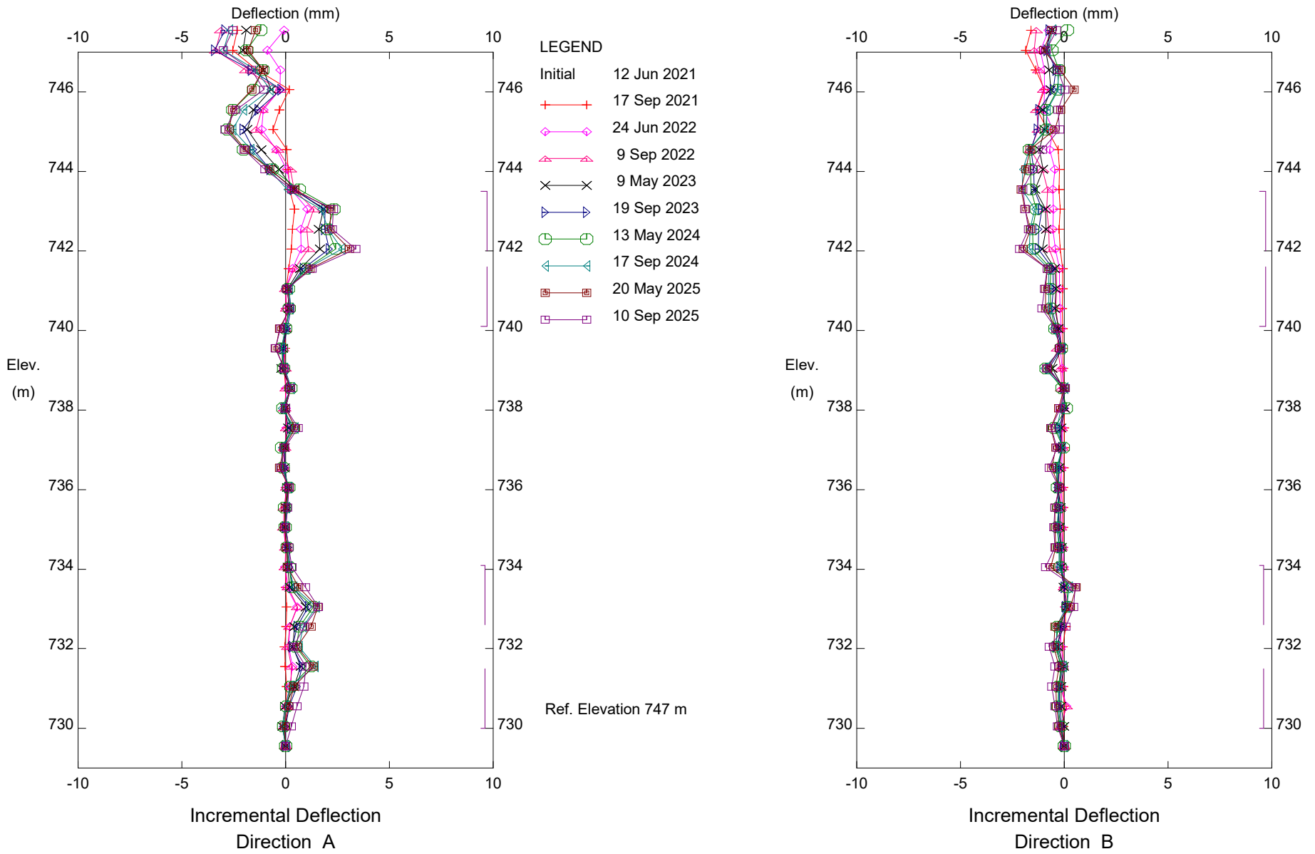
C017-III; H575:04; Truckstop Slide, Inclinometer SI20-01 Alberta Transportation
